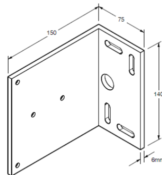
HM 130 00 mounting bracket
