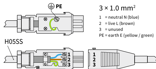
connecting plug (Hirschmann STAK3 connector)
