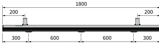
markilux spotline LED with 3 spotlights and 2 brackets
