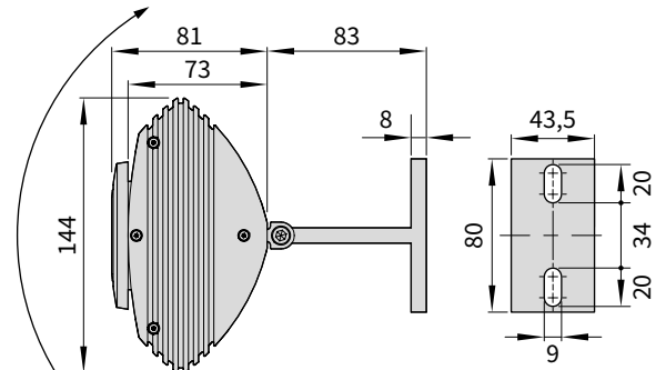
side view of the markilux spotline LED illustrating face fixture dimensions in mm
