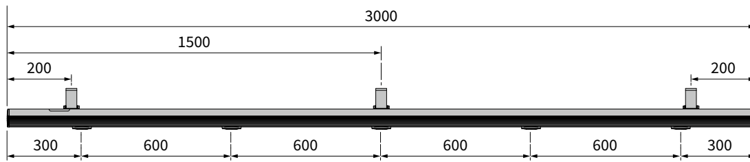
markilux spotline LED with 5 spotlights and 3 brackets
