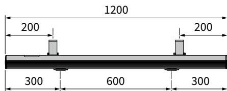
markilux spotline LED with 2 spotlights and 2 brackets
