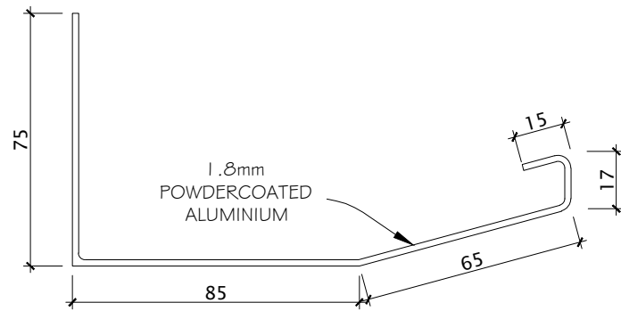
GUTTER SECTION SCALE 1:2
