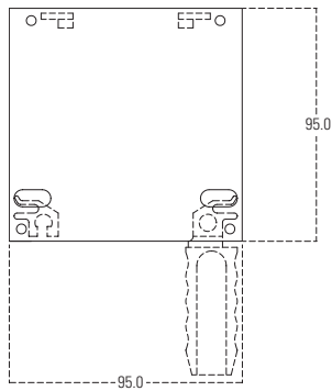
70mm HEADBOX END CAP
